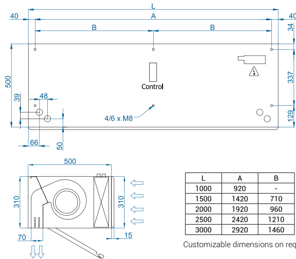
Horizontal installation
