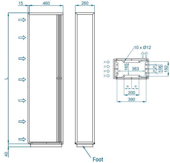
Vertical installation
