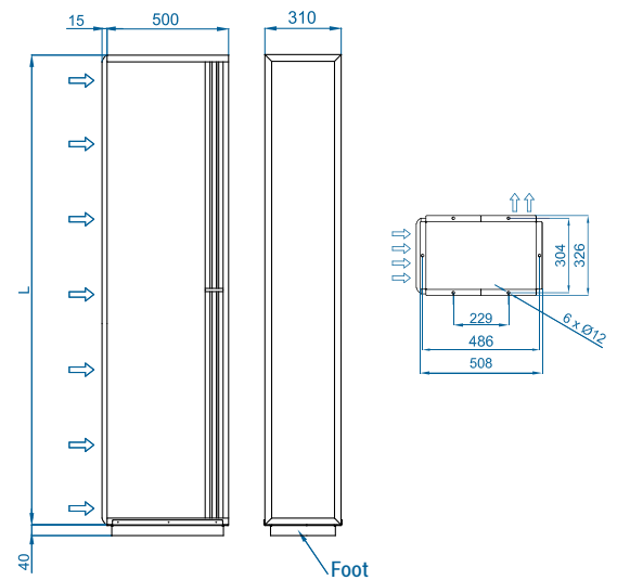
Vertical installation
