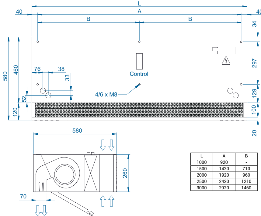
Horizontal installation
