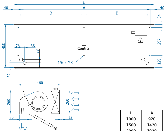
Horizontal installation
