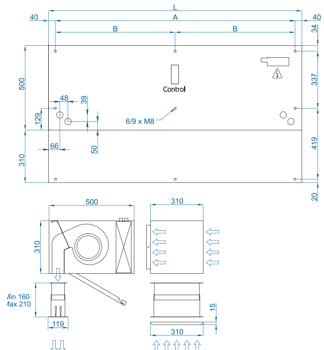
False ceiling invisible mounting
